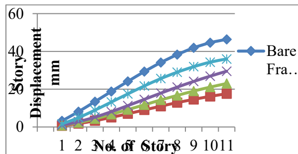
Story Drift in Y Direction for G+11 in Z=0.1
