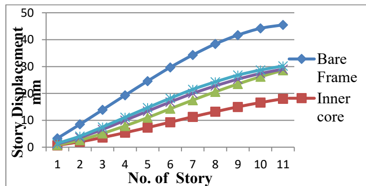
Displacement in Y Direction for G+11 in Z=0.1
